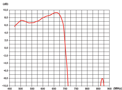
Gain curve Phoenix
